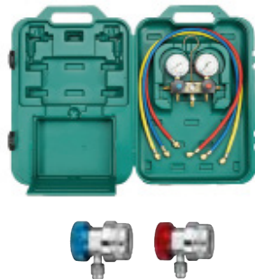
AMS450-077 Manifold With Two Taps And Three Hoses For R134a/R404a (including Quick Connections)
