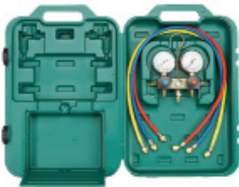
AMS450-009 Manifold With Two Taps And Three Hoses For R134a/R404a
