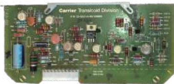
Temperature Control Board, Repaired AC12-00214-XX
