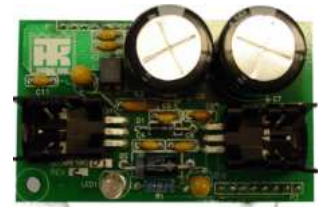
Spectrum TS Power Supply Board, Repaired AT41-4096
